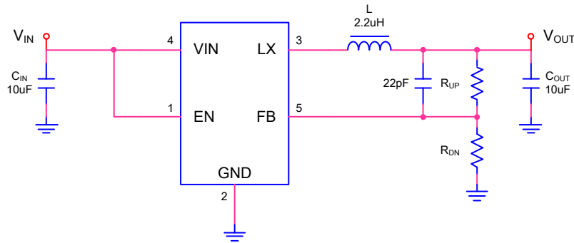
Adjustable Voltage Application Circuit
