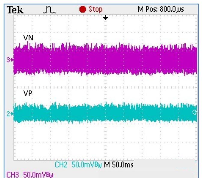
V_{in}=3.3\text{V}, C_{out}=2.2\mu\text{F}, I_{VP}=I_{VN}=50\text{mA}
