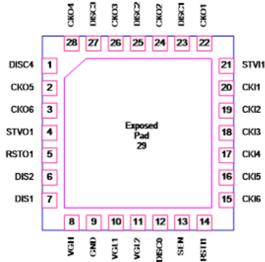
Figure 2. QFN-28 Package (4mm x 4mm)
