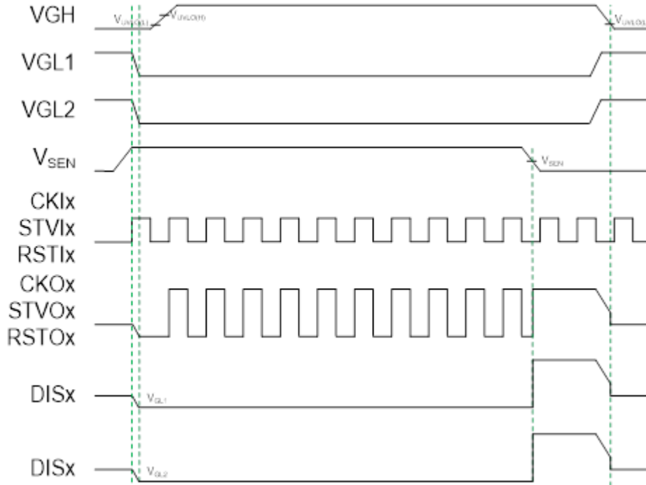
Figure 4. Power Sequence with TCON Mode
