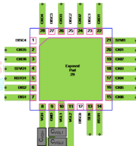
Figure 6. Recommended LP6297A PCB Layout
