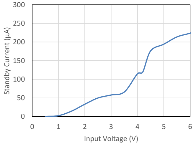
Figure 2. Input Standby Current vs Input Voltage Charge terminated, 25^{\circ}C
