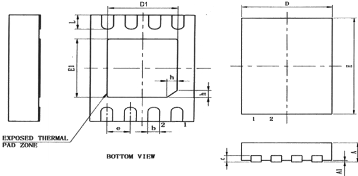
DFN-8
