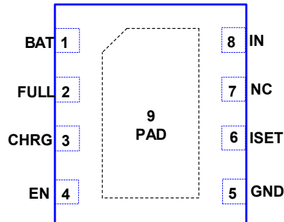
DFN-8 (Top View)
