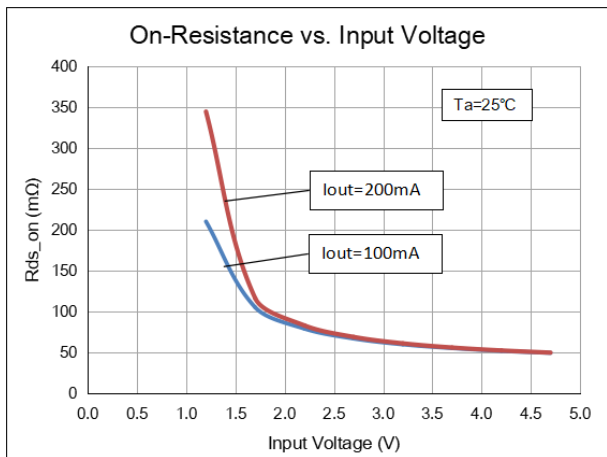
Figure 6 R_{ON} vs Voltage ( C_{IN}=C_{OUT}=1\mu F , T_A=25^\circ C )
