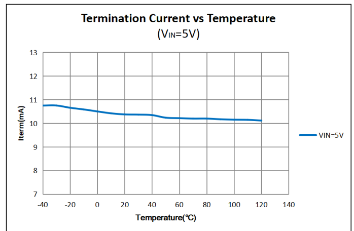
Figure 5. Termination Current vs Temperature ( C_{IN}=10\mu F , C_{OUT}=22\mu F , R_{ISET}=16k\Omega )
