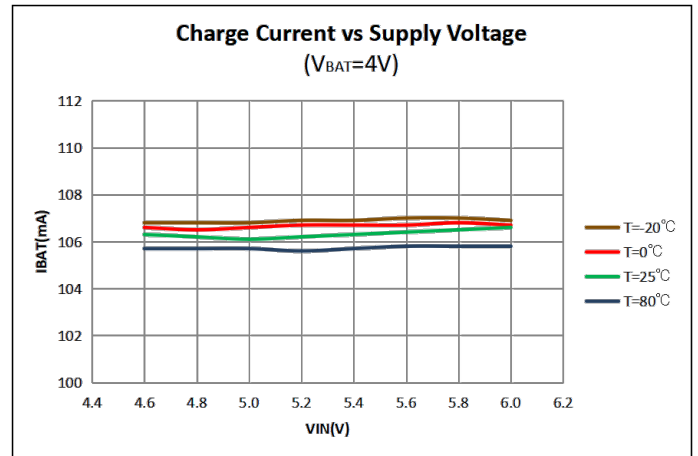
Figure 3. Charge Current vs Supply Voltage ( C_{IN}=10\mu F , C_{OUT}=22\mu F , R_{ISET}=16k\Omega )
