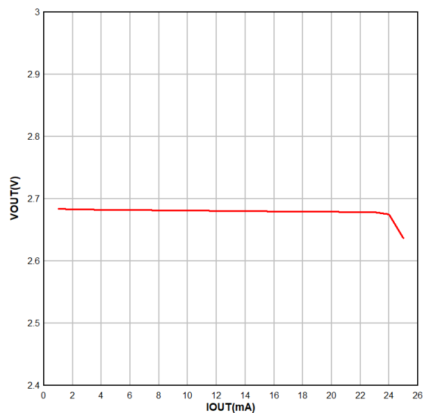
Figure 24. LDO load regulation
