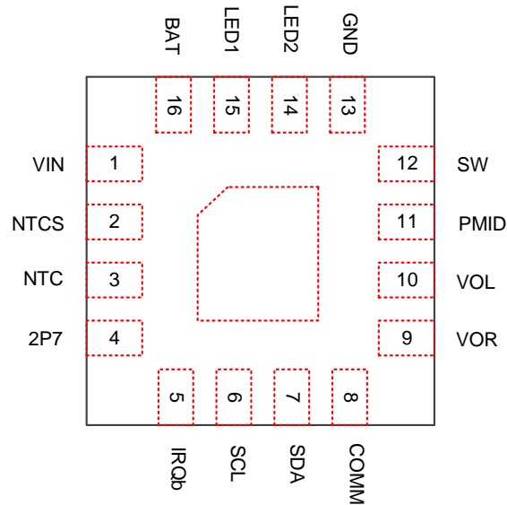
LP7810 Pinout
