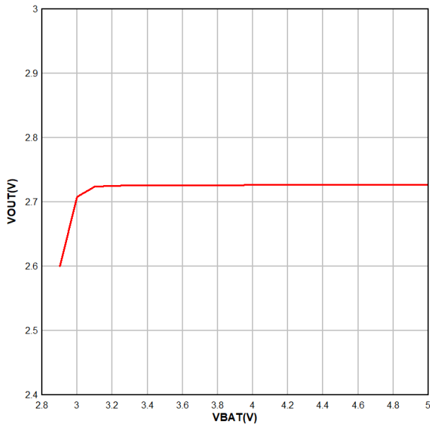
Figure 23. LDO line regulation
