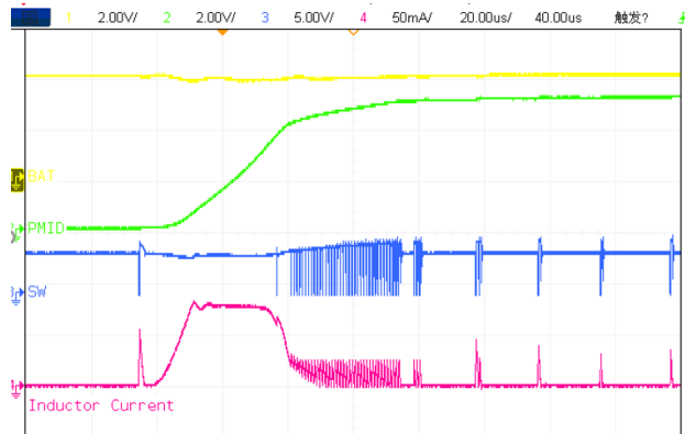
Figure 17. Startup waveform, VIN=4.0V, no load
