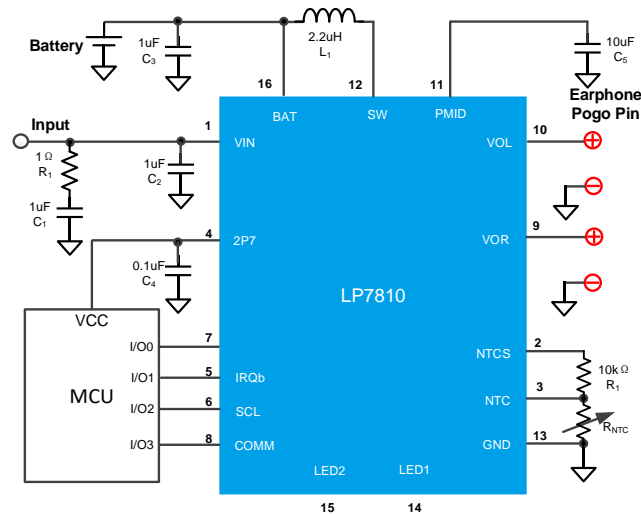
Figure 14. Typical Application circuit
