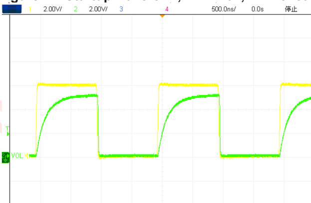
Figure 19. VOL UART TX, 1.5Mbps, and COMM
