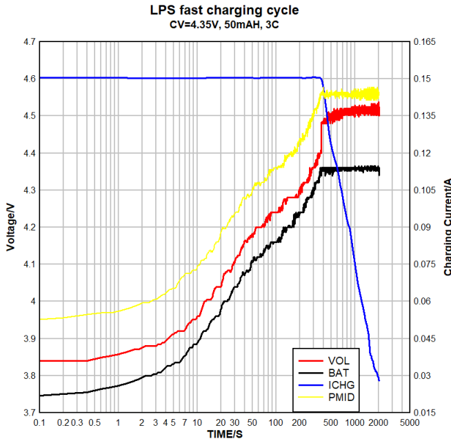
Figure 21. Charging Cycle, Case=3.6V LDO line regulation IOUT=15mA
