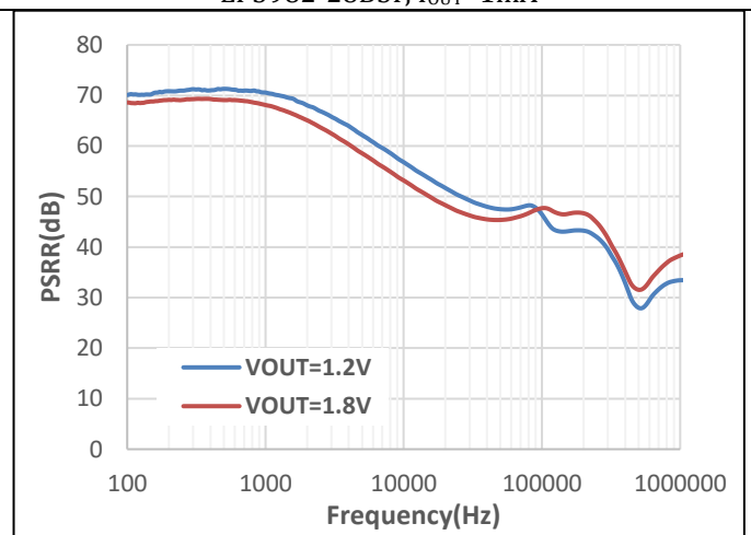
Figure 6. PSRR vs Frequency with V_{OUT}=1.2\text{V}/1.8\text{V}
