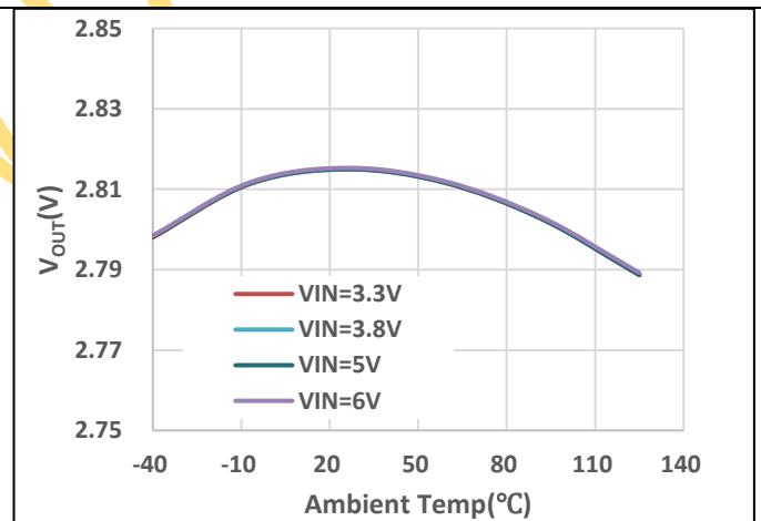
Figure 4. V_{OUT} vs Ambient Temperature, LP3982-28B5F, I_{OUT}=1\text{mA}
