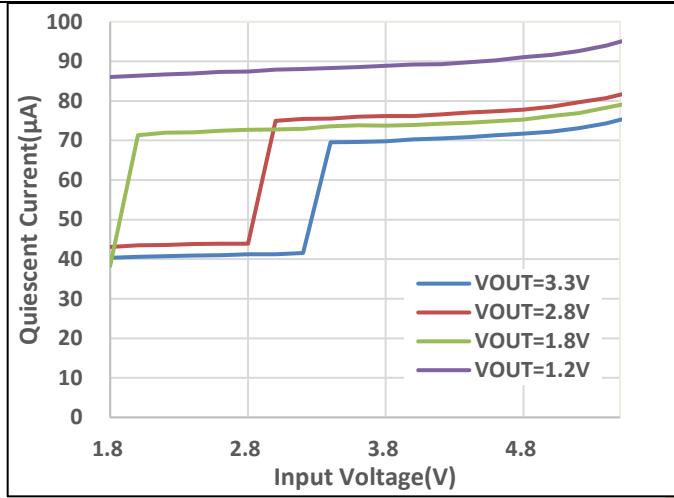
Figure 1. Quiescent current vs input voltage, 25°C
