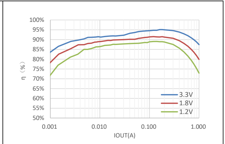
Figure 2 Efficiency with V_{IN}=5V @ Different Load
