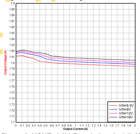
Figure 8. VOUT=1.8V, Regulation, L=1.5uH
