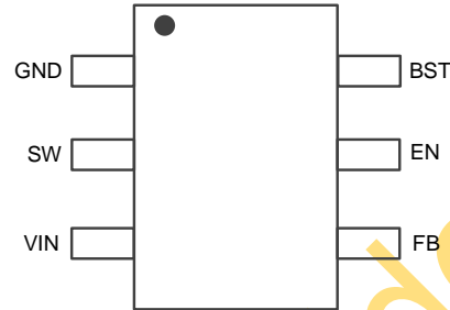
SOT23-6 (Top View) LP6450AT
