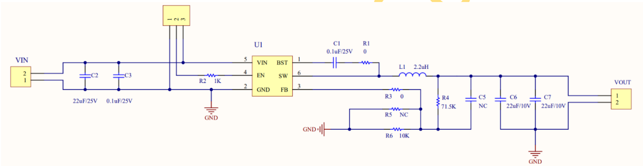
Figure 28. Typical schematic
