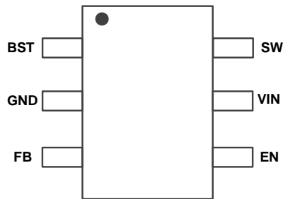
SOT23-6 (Top View) LP6450A
