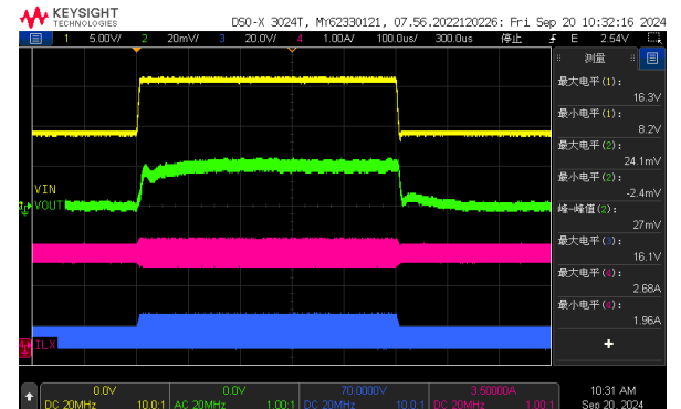
Figure 21. Line Transient, 2A load
