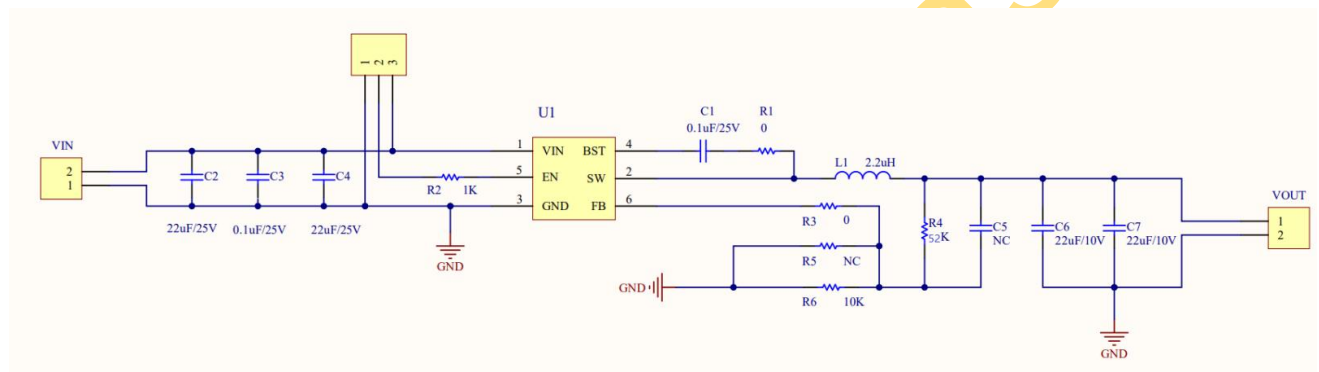
Figure 10. Typical schematic
