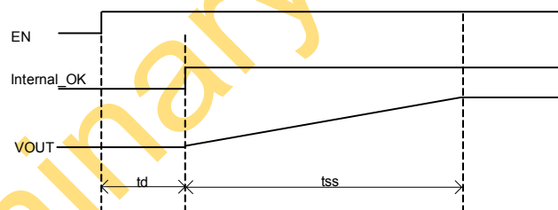
Figure 9. Soft Start Sequence
