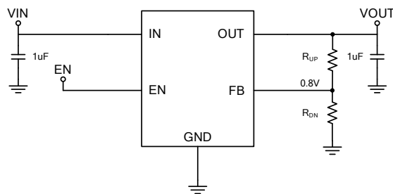
Adjustable Voltage Application Circuit
