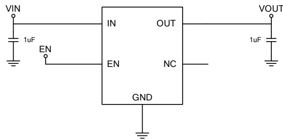
Fixed Voltage Application Circuit
