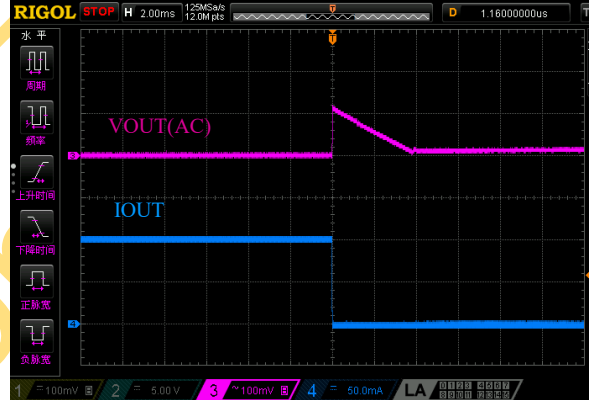
Figure 18 Load Transient I_{OUT}=100\text{mA}\rightarrow 1\text{mA} with V_{IN}=12\text{V}
