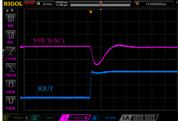
Figure 17 Load Transient I_{OUT}=1\text{mA}\rightarrow 100\text{mA} with V_{IN}=12\text{V}
