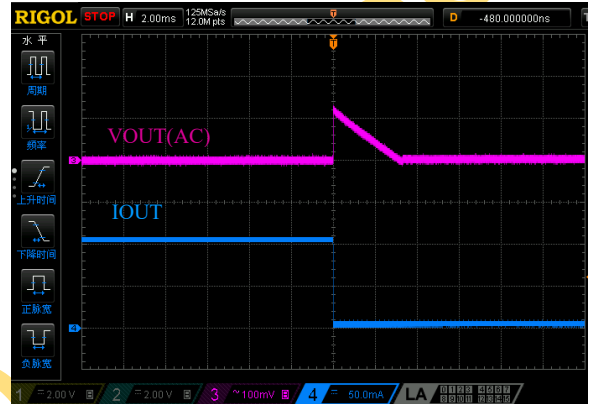
Figure 16 Load Transient I_{OUT}=100\text{mA}\rightarrow 1\text{mA} with V_{IN}=5\text{V}
