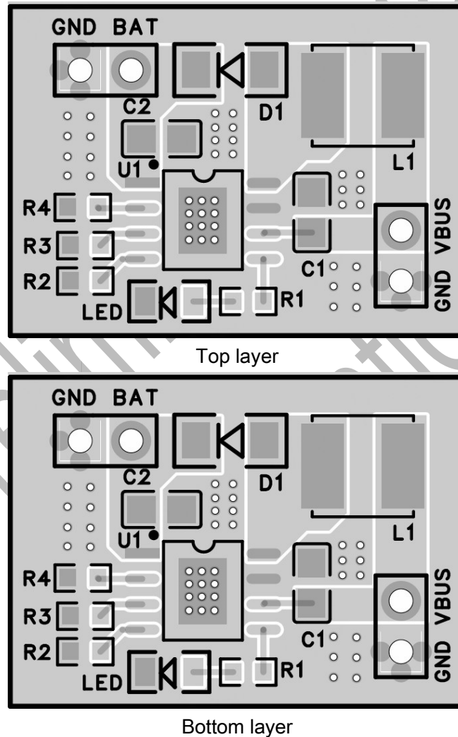
Figure 3. 2-layer PCB layout example
