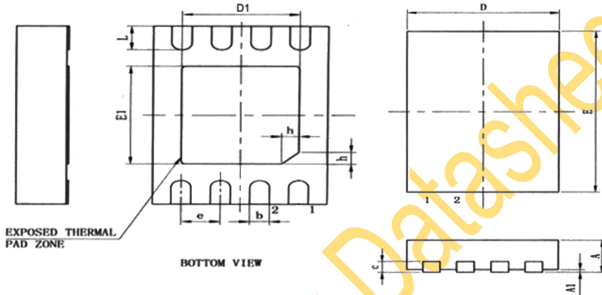
DFN3x3mm-8
