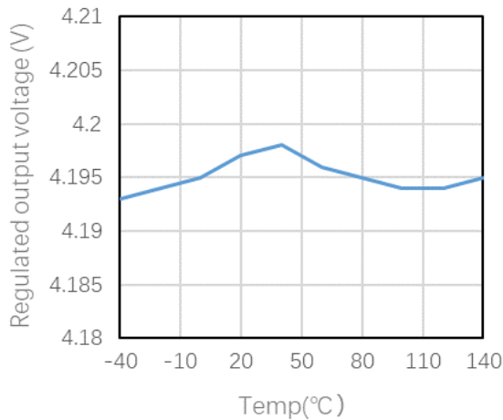
Figure 5. Regulated Output Voltage ( V_{FLOAT} ) vs Ambient Temperature
