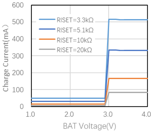
Figure 1. Charge Current vs BAT Voltage V_{IN}=5V , 25^{\circ}C
