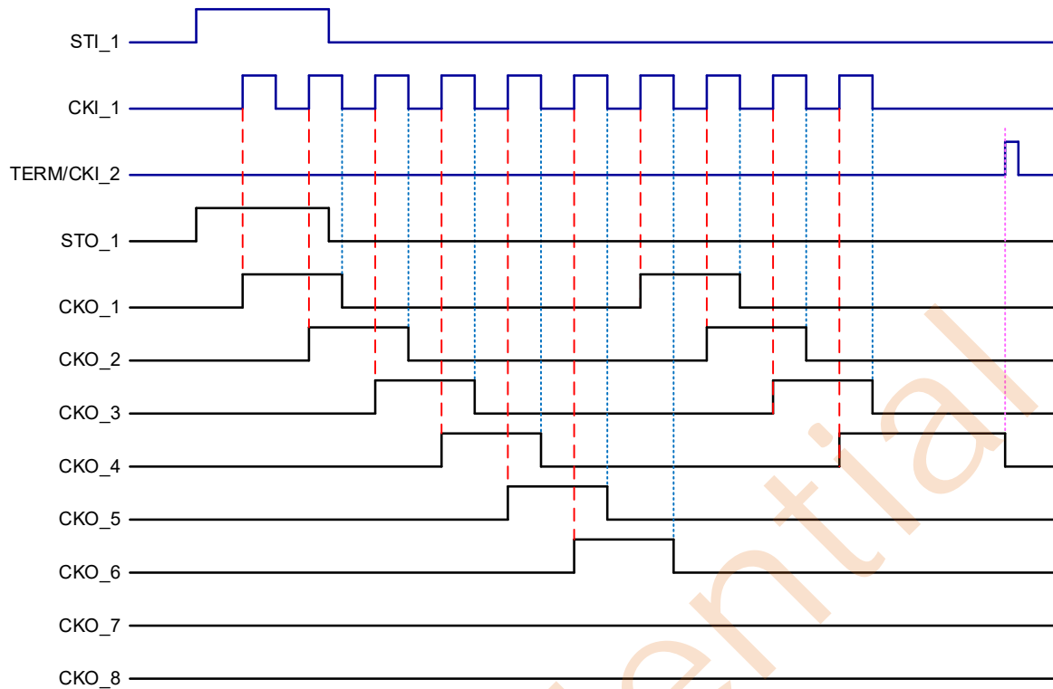
SET3=Low: 1 input mode ; SET1=Low: 6 phase
