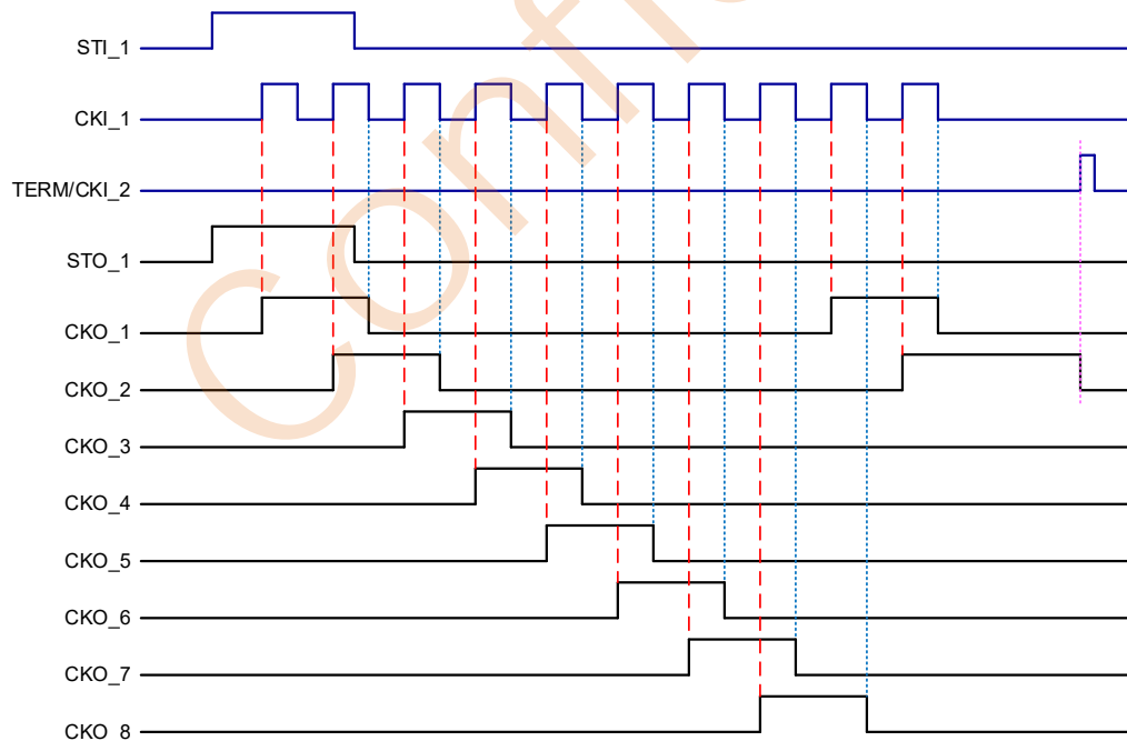
SET3=Low: 1 input mode ; SET1=High: 8 phase
