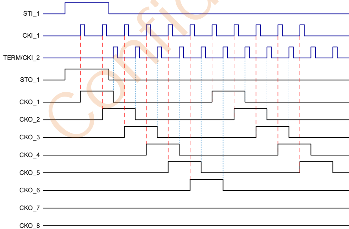
SET3=High: 2 input mode ; SET1=Low: 6 phase
