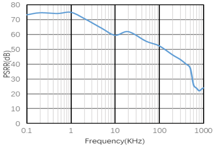
Figure 3 PSRR vs Frequency V_{OUT}=3.3\text{V}
