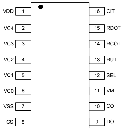
SSOP16 (top view)
