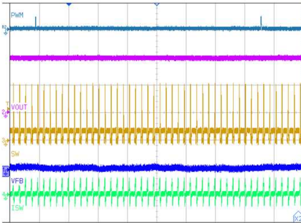
Figure 26. Steady state ( V_{IN}=3.7V , PWM Dimming Duty = 0.25%)
