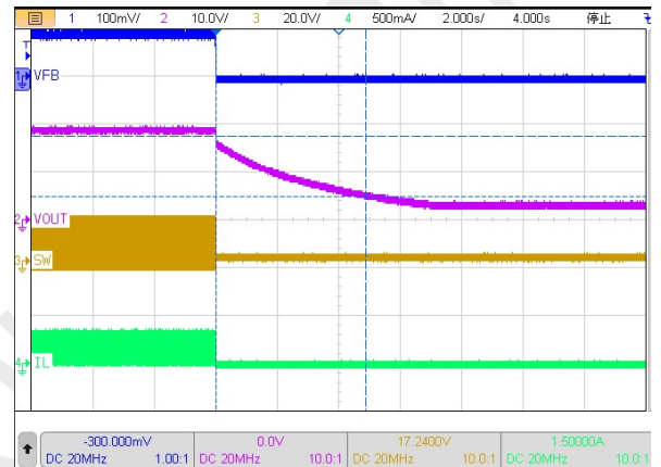
Figure 19. Shutdown ( V_{IN}=3.7V , PWM Dimming Duty = 40%)
