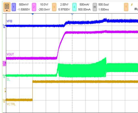
Figure 16. Startup ( V_{IN}=3.7V , PWM Dimming Duty = 100%)
