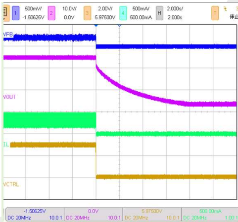
Figure 18. Shutdown ( V_{IN}=3.7V , PWM Dimming Duty = 100%)
