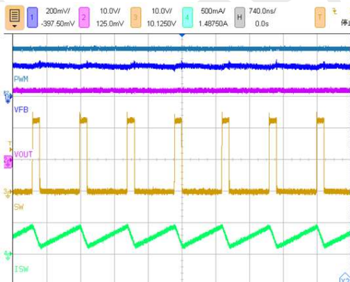
Figure 20. Steady state ( V_{IN}=3.7V , PWM Dimming Duty = 100%)
