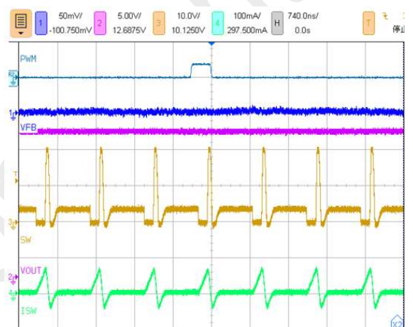
Figure 25. Steady state
