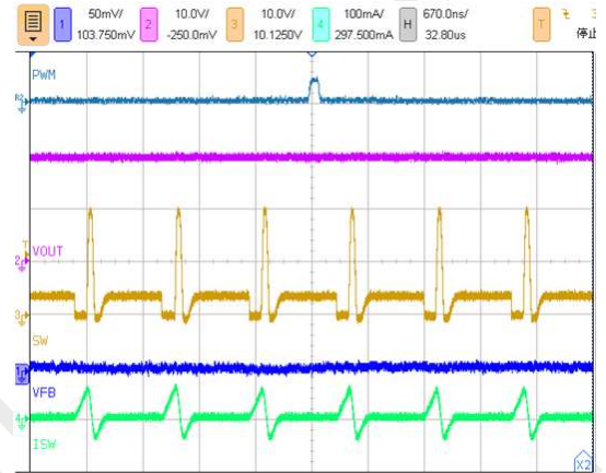
Figure 27. Steady state ( V_{IN}=3.7V , PWM Dimming Duty = 0.25%)
