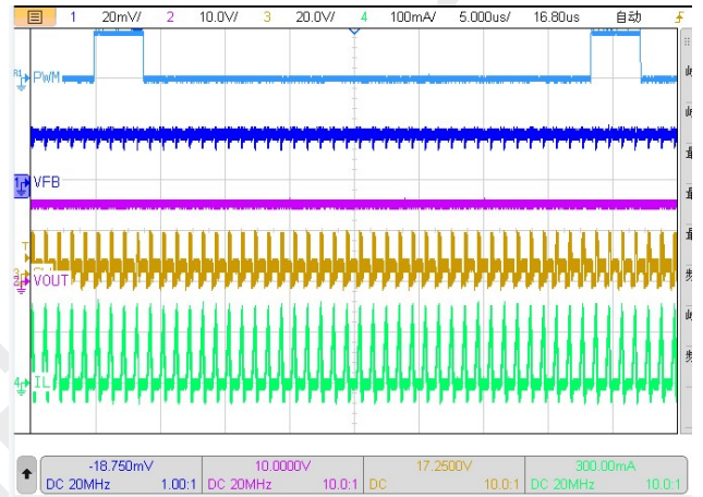
Figure 23. Steady state
