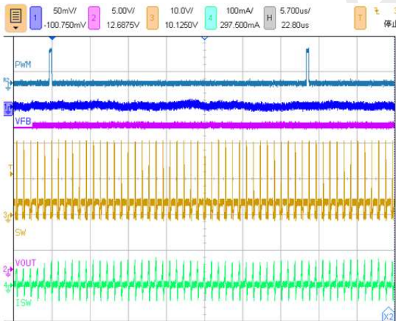
Figure 24. Steady state
