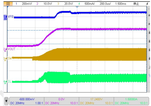
Figure 17. Startup ( V_{IN}=3.7V , PWM Dimming Duty = 40%)
