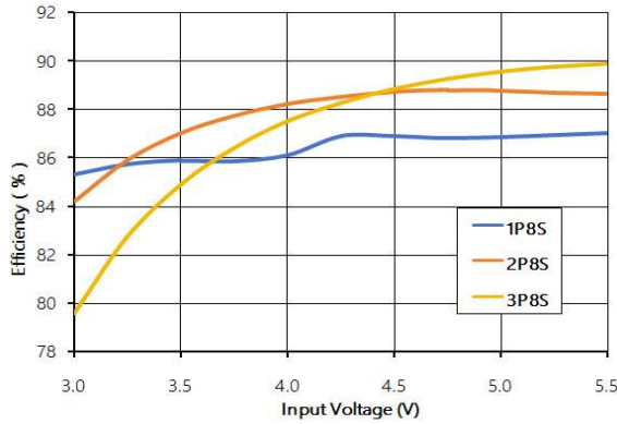
Figure 1. Efficiency vs. Input Voltage (L1: 2.5mmx2.0mmx1.2mm, DCR=480mΩ)
