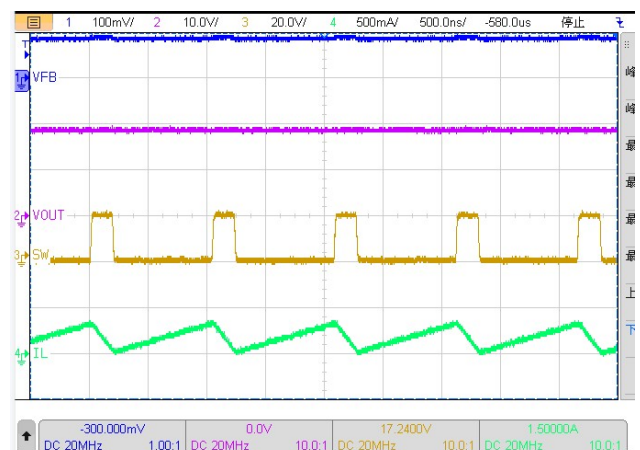
Figure 21. Steady state ( V_{IN}=3.7V , PWM Dimming Duty = 40%)
