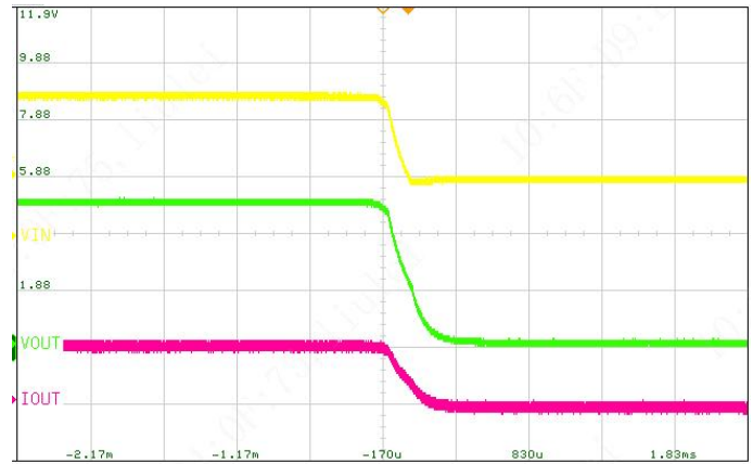
Figure 7. Shut-down Relative to V_{IN} ( C_{IN}=C_{OUT}=1\mu F , R_{LOAD} = 100\Omega )
