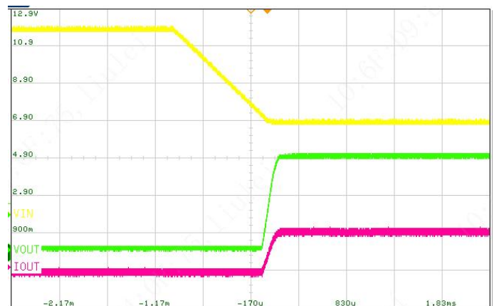
Figure 9. Over-Voltage Protection Recovery ( V_{IN} from 10V to 5V, C_{IN}=C_{OUT}=1\mu F , R_{LOAD} = 100\Omega )
