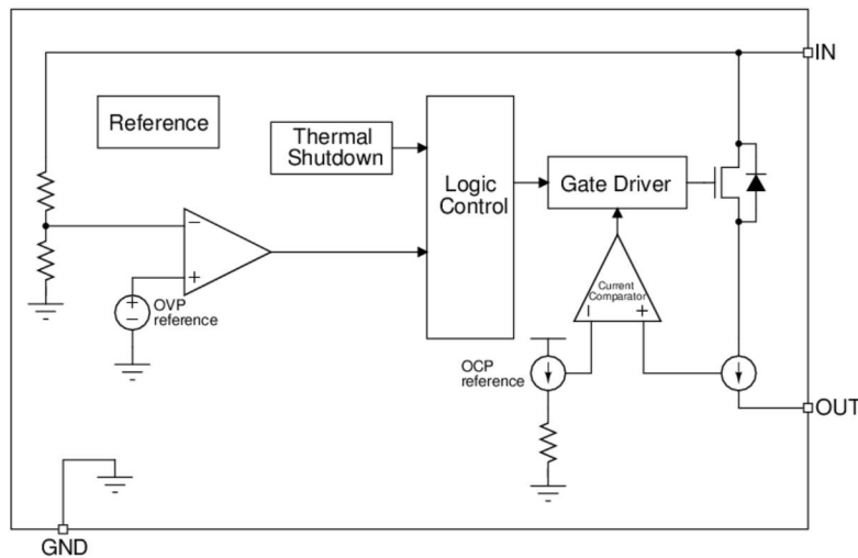
Figure 2. Internal Block Diagram (LP5313)
