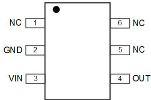
SOT23-6 (Top View)
