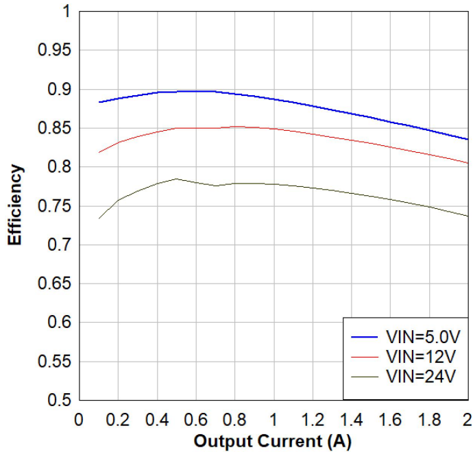
Figure 3. V_{OUT}=1.8V , Efficiency, L=1\text{-}\mu\text{H} , LP6432H
