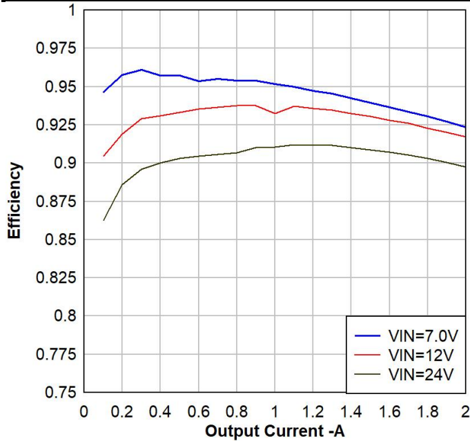
Figure 9. V_{OUT}=5.0V , Efficiency, L=4.7-\mu H , LP6432
