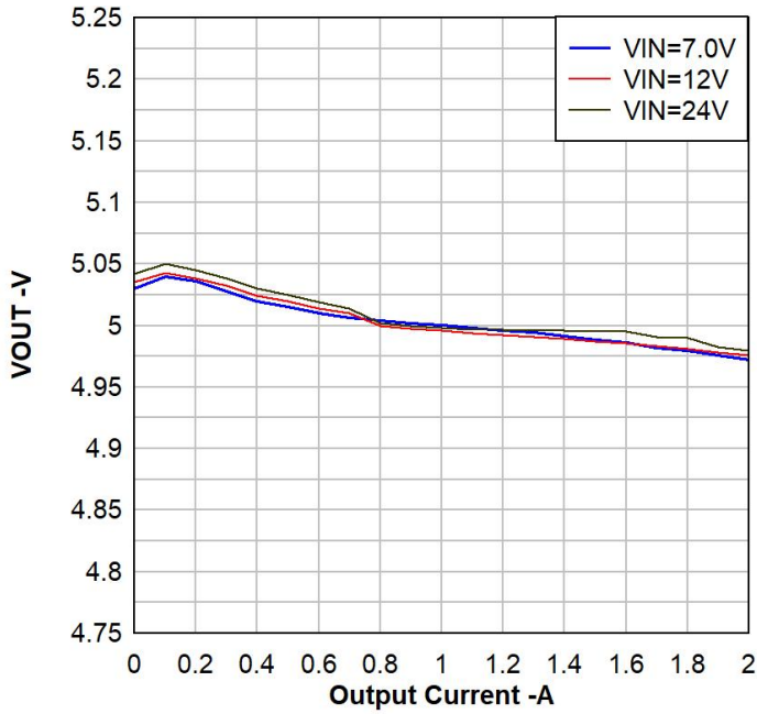
Figure 5. VOUT=5V, Regulation, L=4.7- \mu H, LP6432H
