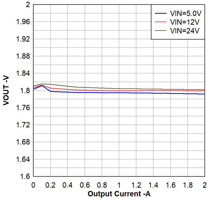
Figure 7. VOUT=1.8V, Regulation, L=1- \mu H, LP6432H
