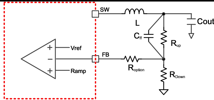
Figure 33. FB connection
