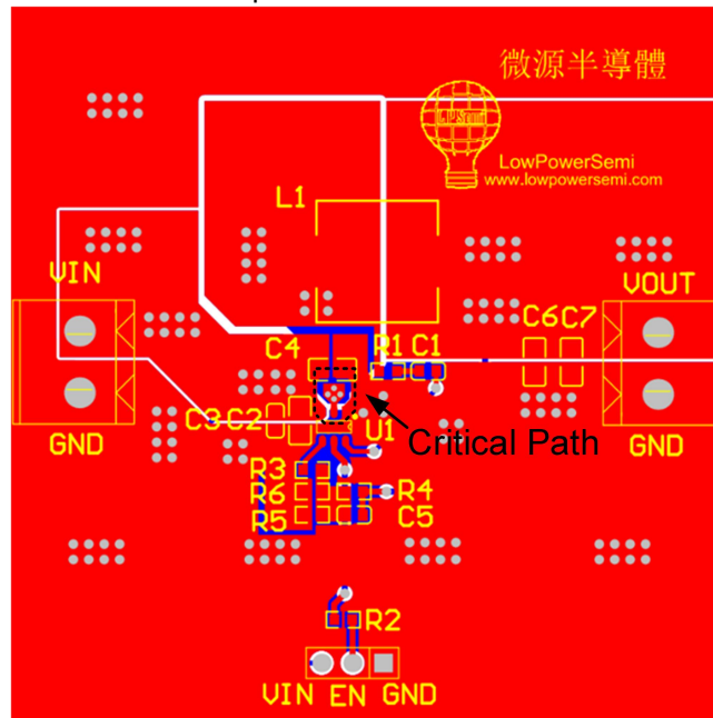
Figure 35 Layout example
