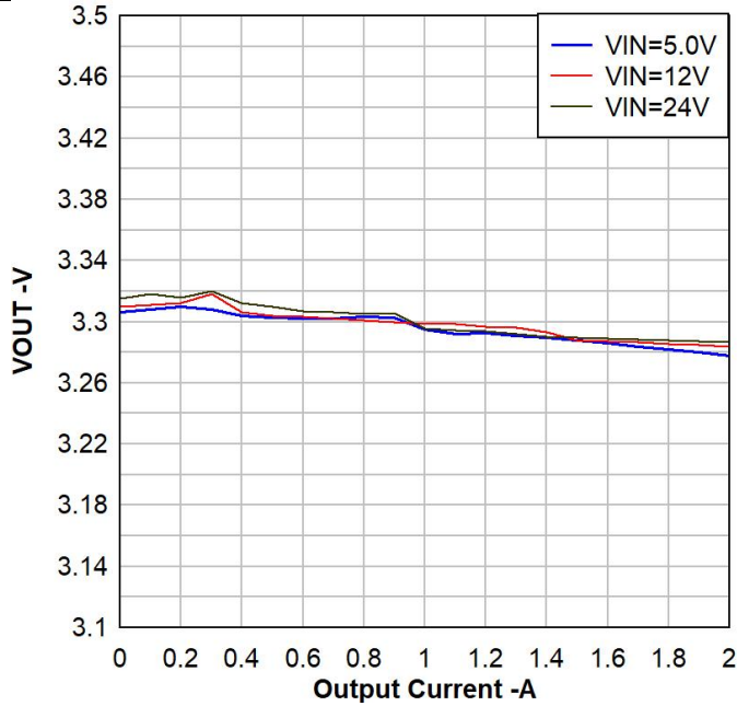
Figure 13. V OUT =3.3V, Regulation, L=4.7- \mu H, LP6432
