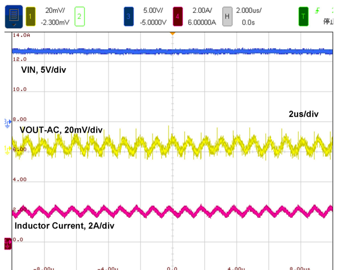
Figure 26. Switching Waveform, 2A load
