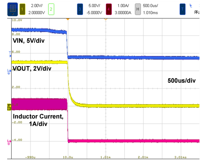
Figure 18. Shutdown by VIN, 2.5Ω load
