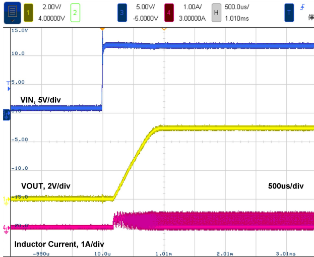
Figure 15. Startup by VIN, 50Ω load
