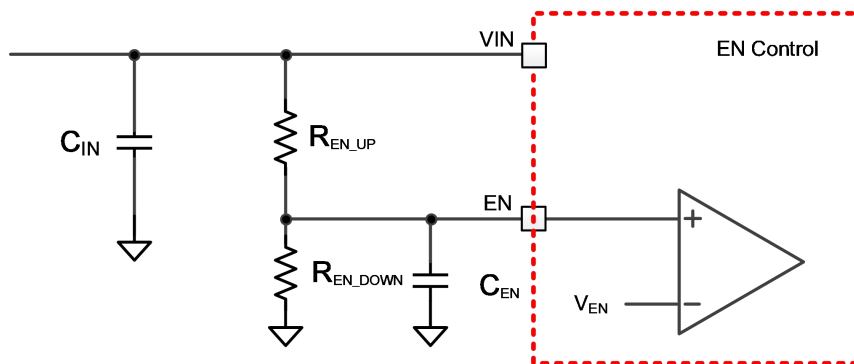
Figure 34. EN connection
