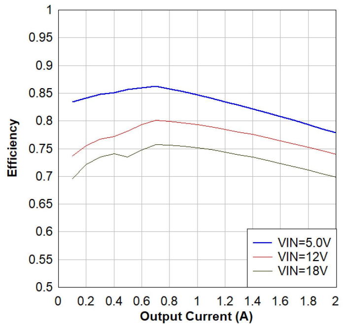
Figure 4. V_{OUT}=1.2V , Efficiency, L=1\text{-}\mu\text{H} , LP6432H
