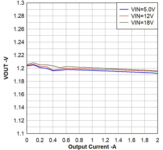
Figure 8. VOUT=1.2V, Regulation, L=1- \mu H, LP6432H
