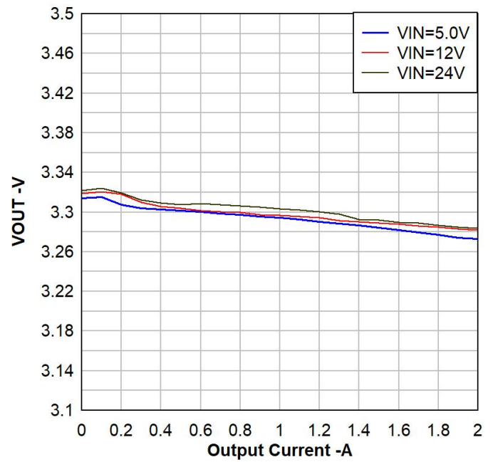
Figure 6. VOUT=3.3V, Regulation, L=3.3- \mu H, LP6432H
