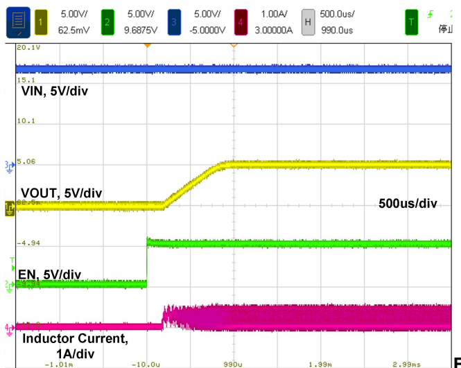
Figure 19. Startup by EN, 50Ω load
