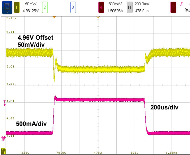
Figure 27. Load Transient, 0.1A-1A-0.1A
