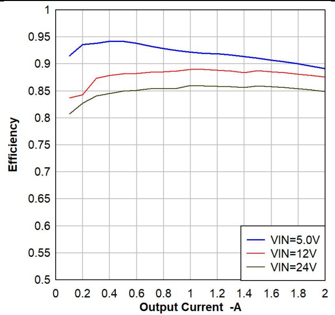
Figure 10. V_{OUT}=3.3V , Efficiency, L=4.7-\mu H , LP6432
