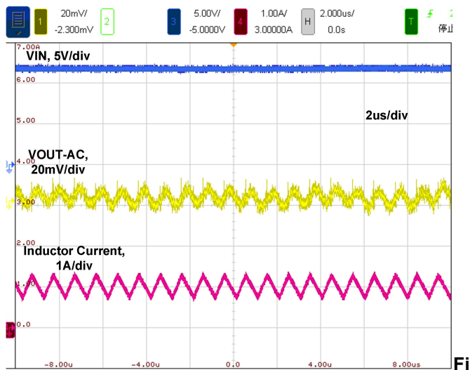
Figure 25. Switching Waveform, 1A load
