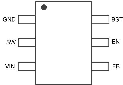
SOT23-6 (Top View) LP6432 Pinout
