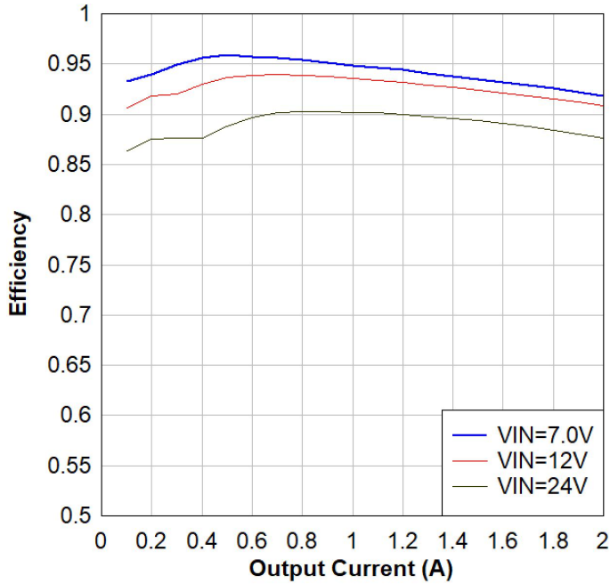
Figure 1. V_{OUT}=5V , Efficiency, L=4.7\text{-}\mu\text{H} , LP6432H
