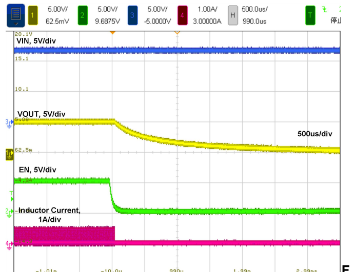
Figure 20. Shutdown by EN, 50Ω load
