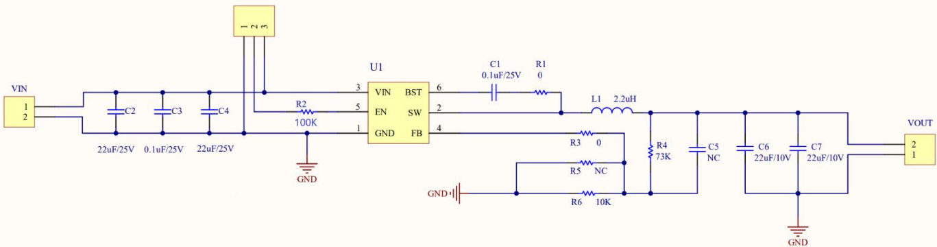
Figure 32. Typical schematic
