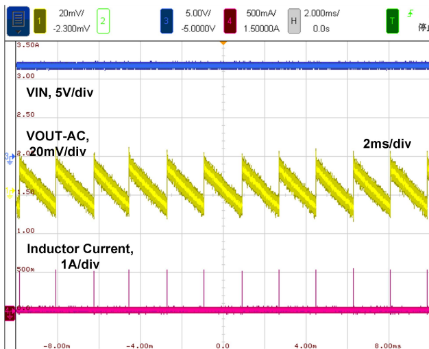
Figure 23. Switching Waveform, 0A load
