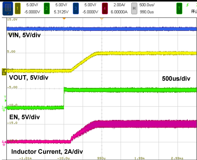
Figure 21. Startup by EN, 2.5Ω load
