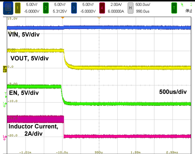
Figure 22. Shutdown by EN, 2.5Ω load
