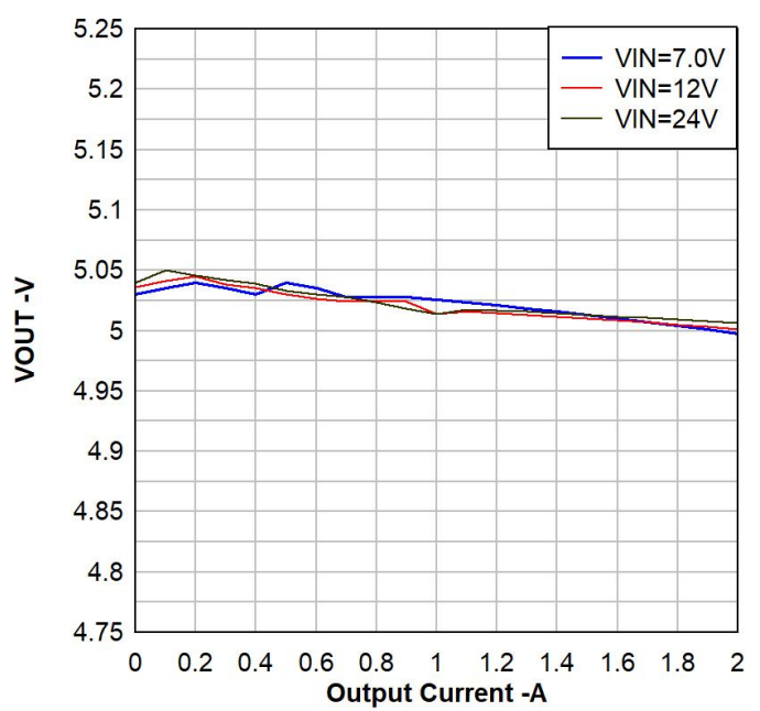
Figure 12. V_{OUT}=5V , Regulation, L=4.7-\mu H , LP6432
