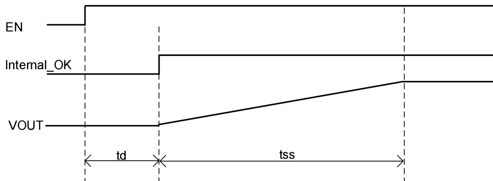
Figure 31. Soft Start Sequence
