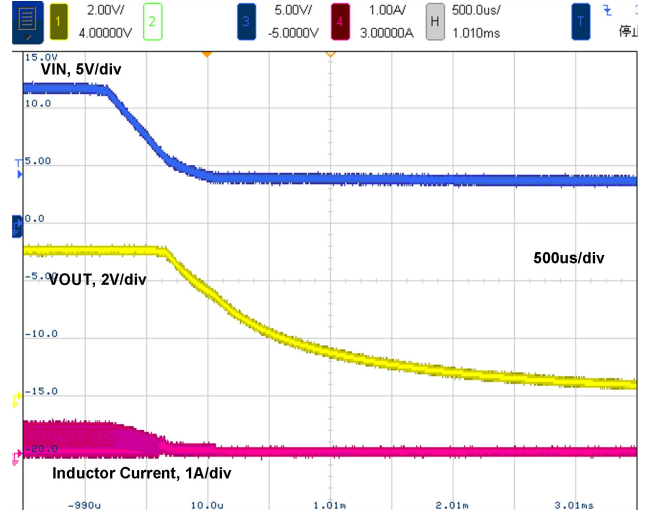
Figure 16. Shutdown by VIN, 50Ω load
