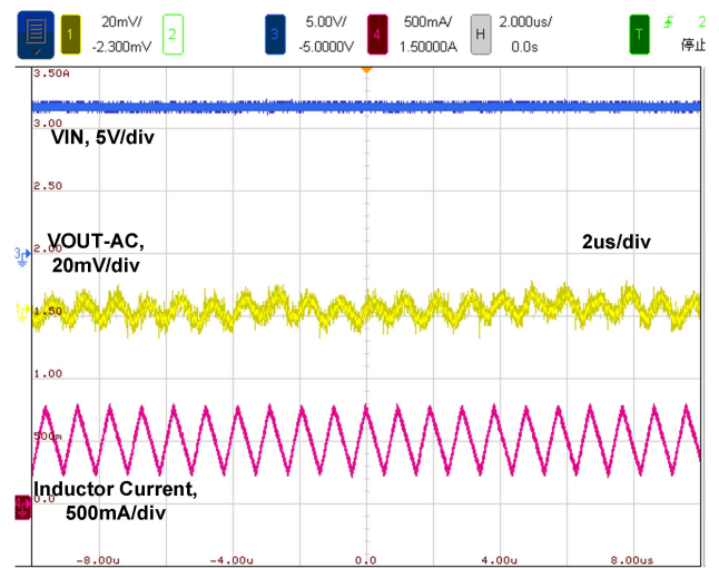
Figure 24. Switching Waveform, 500mA load
