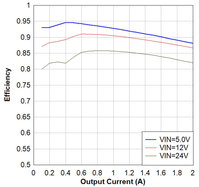
Figure 2. V_{OUT}=3.3V , Efficiency, L=3.3\text{-}\mu\text{H} , LP6432H
