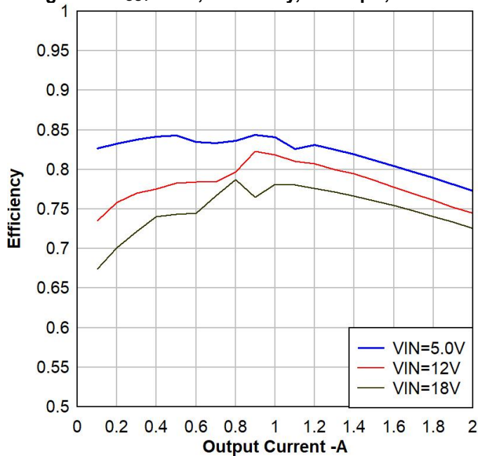
Figure 11. V_{OUT}=1.2V , Efficiency, L=2.2-\mu H , LP6432
