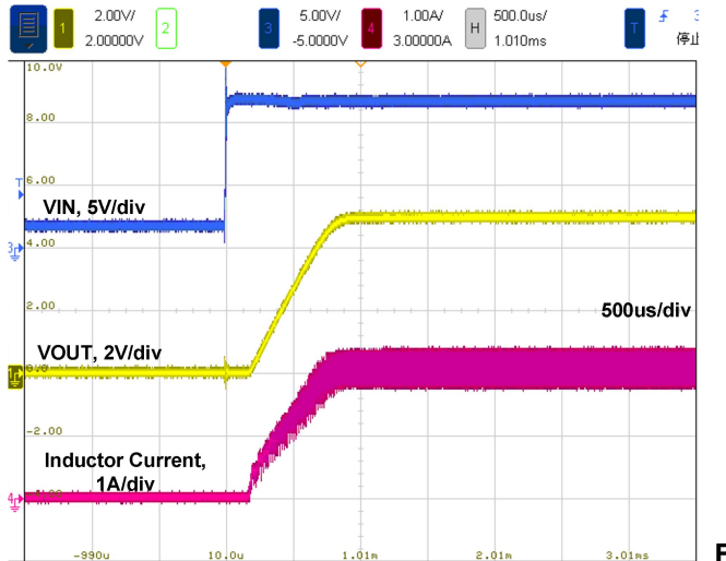
Figure 17. Startup by VIN, 2.5Ω load
