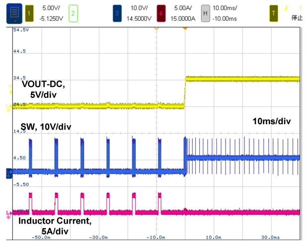
Figure 30. SCP Recovery
