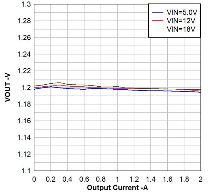
Figure 14. V OUT =1.2V, Regulation, L=2.2- \mu H, LP6432
