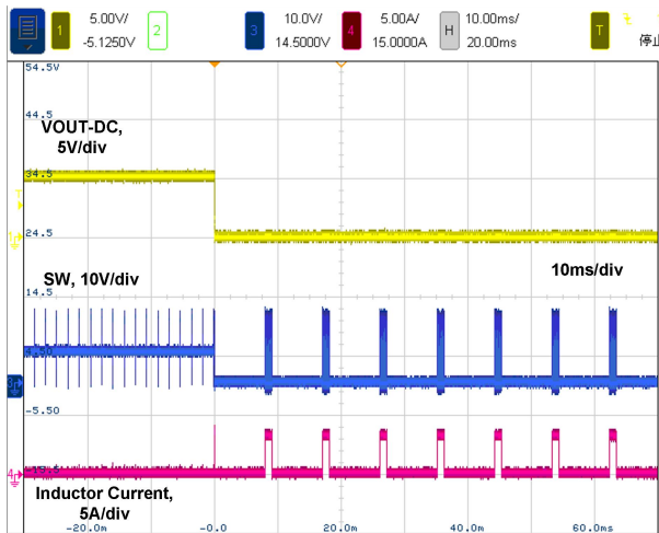
Figure 29. SCP Happen, Hiccup Operation
