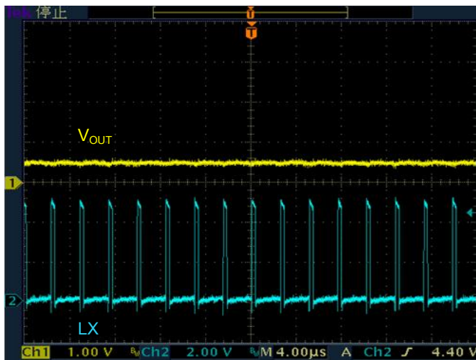
LX waveform @ V_{OUT}=3.3V, \text{Short Output}
