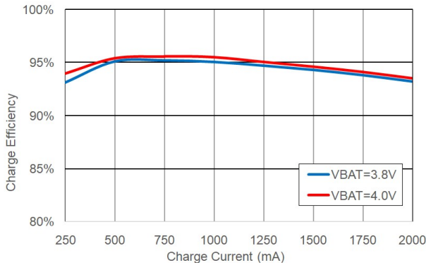
Figure 1. Battery Charge Efficiency (Inductance: L = 1\mu\text{F} , 2.5\text{mm}\times 2.0\text{mm} , \text{DCR}=25\text{m}\Omega )
