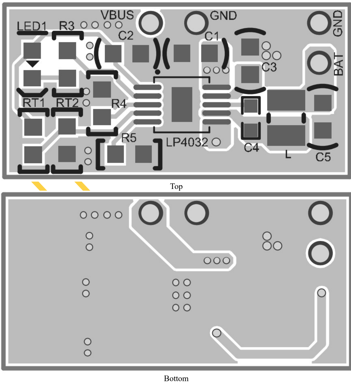
Figure 18. 2-layer PCB Layout Example (20mm x 10mm)
